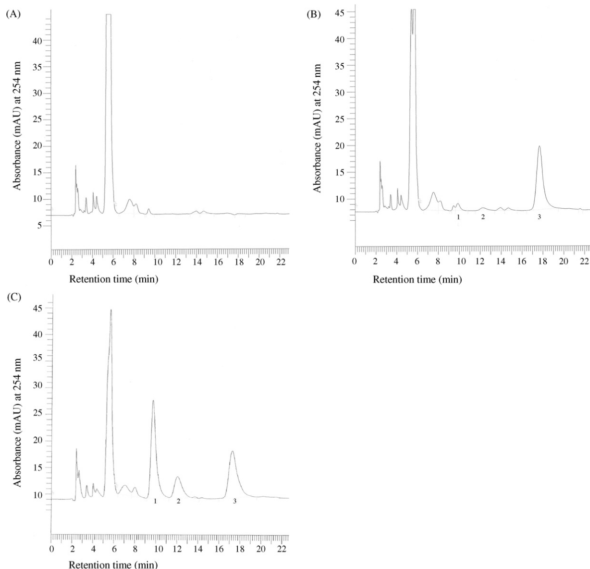
Fig. 1. Chromatogram of analysis of allopurinol and oxipurinol in human serum. Retention times are 9.9 min for oxipurinol (1), 12.3 min for allopurinol (2), and 17.7 min for aciclovir (3; internal standard). (A) Blank pooled human serum; (B) allopurinol 0.5 mg/L and oxipurinol 1.0 mg/L; (C) allopurinol 4.0 mg/L and oxipurinol 20 mg/L.
